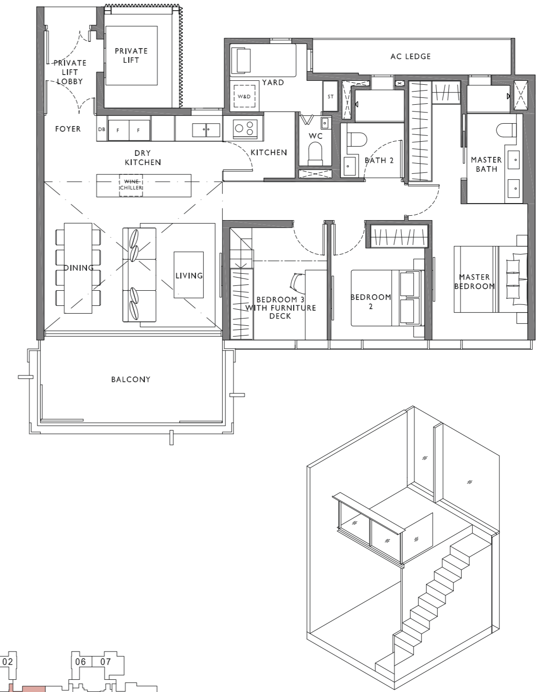
ISOMETRIC VIEW
