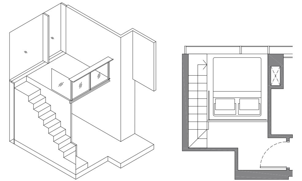
ISOMETRIC VIEW
