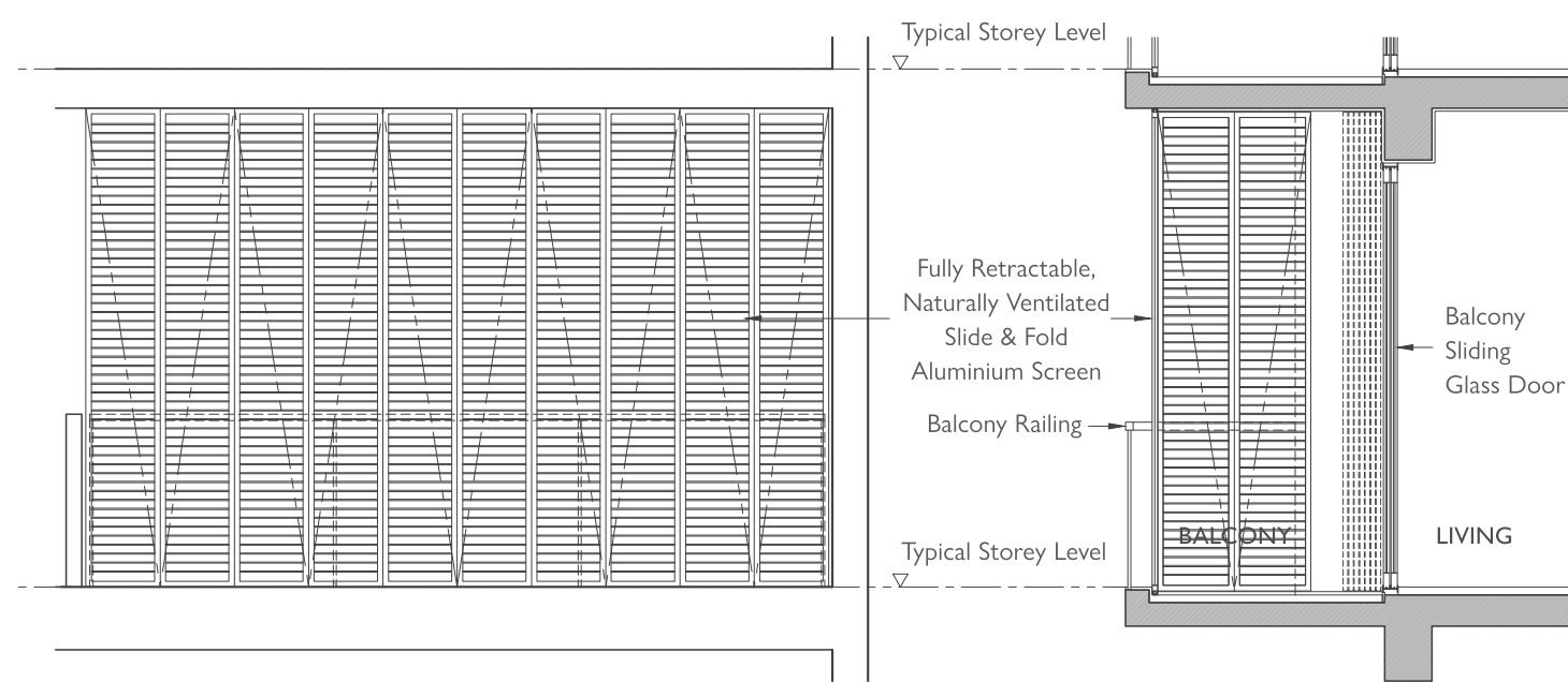
FRONT ELEVATION
