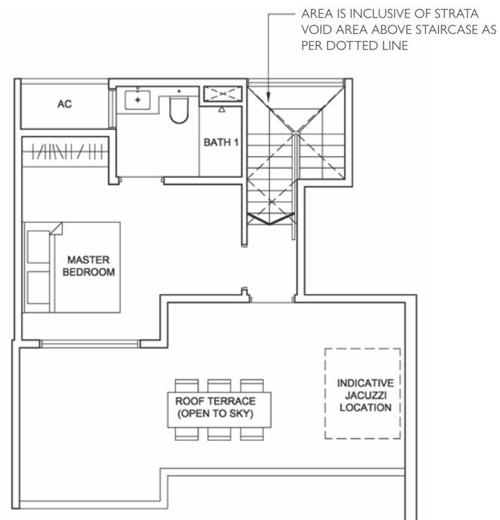
UPPER LEVEL
