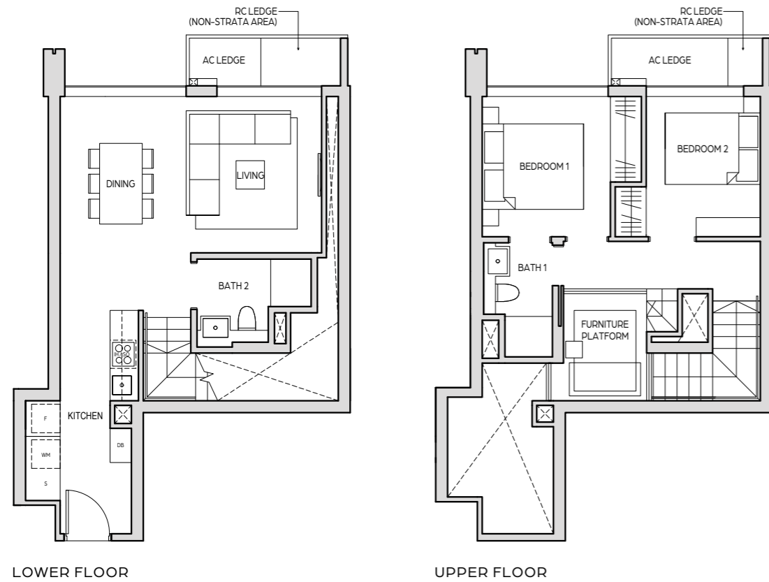
LOWER FLOOR
