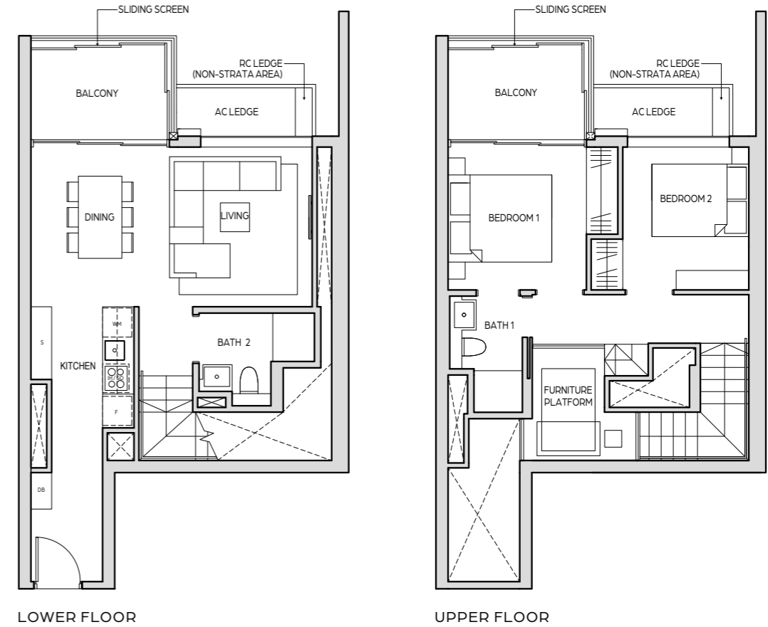
LOWER FLOOR
