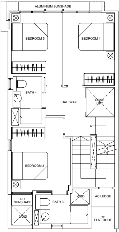
3RD STOREY
