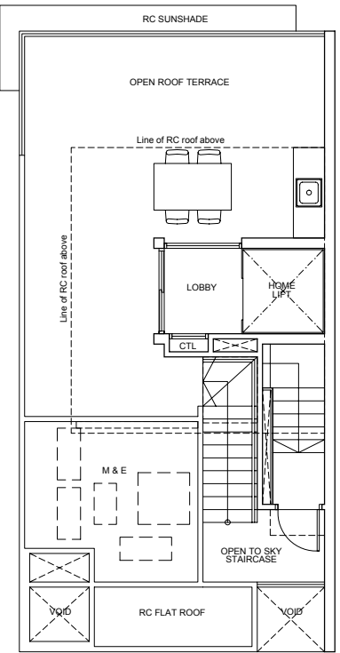
ROOF TERRACE
