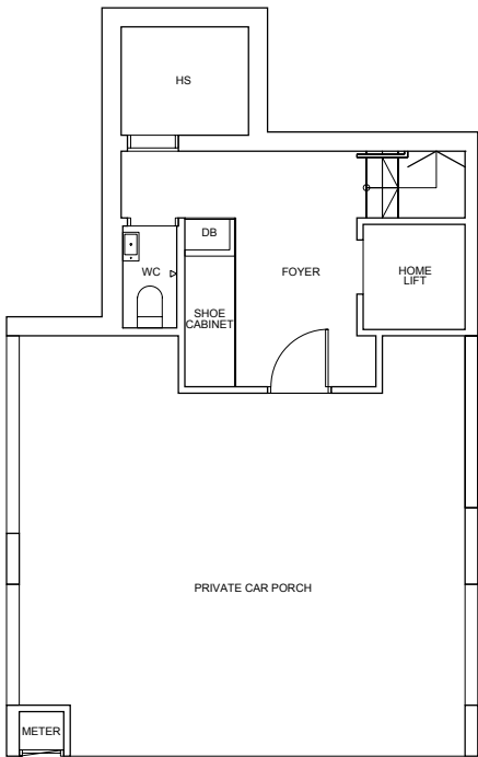
BASEMENT
