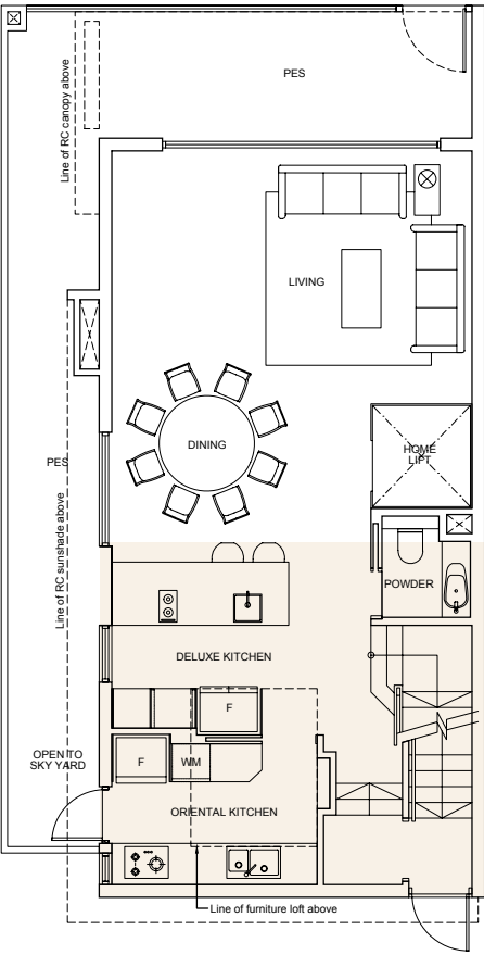
1ST STOREY
