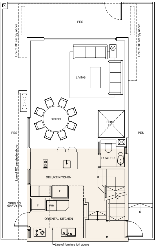
1ST STOREY
